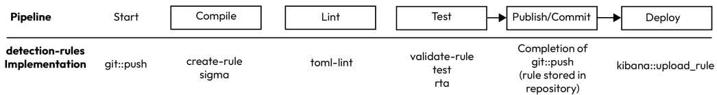
Figure 8.8 – Pipeline with detection-rules implementation
