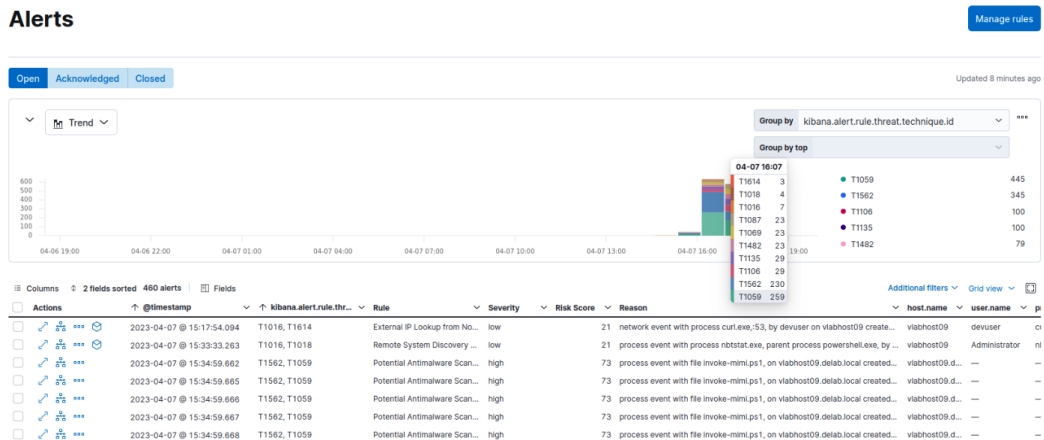
Figure 9.19 – Modified Alerts view in Elastic Security
