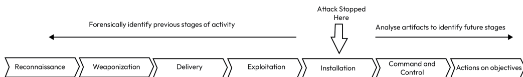
Figure 11.9 – Cyber Kill Chain analysis to identify missed activity
