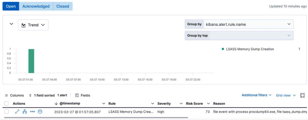
Figure 9.9 – Alerts in the Elastic Security app
