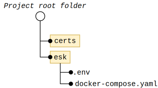
Figure 3.6 – Project folder structure with the Elastic Stack
