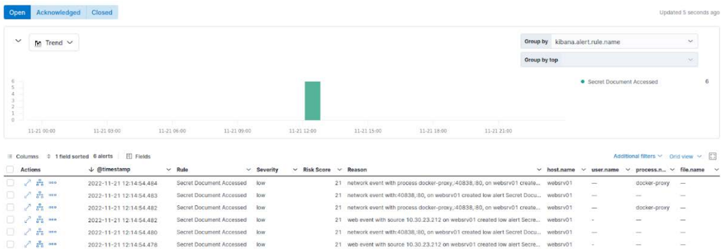
Figure 4.10 – “Secret Document Accessed” alerts
